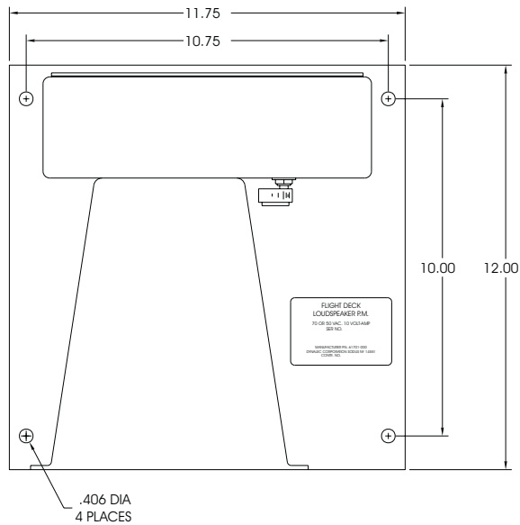
LOUDSPEAKER HEIGHT 8.25"
